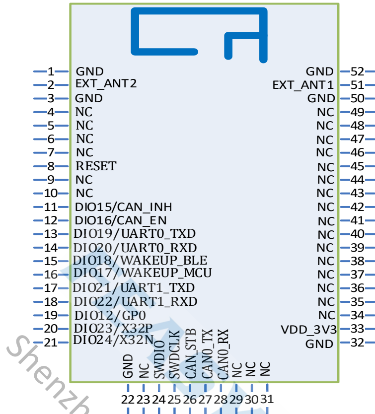
Figure 3-1-2: FSC-BT2004TV PIN Diagram (Top View)
