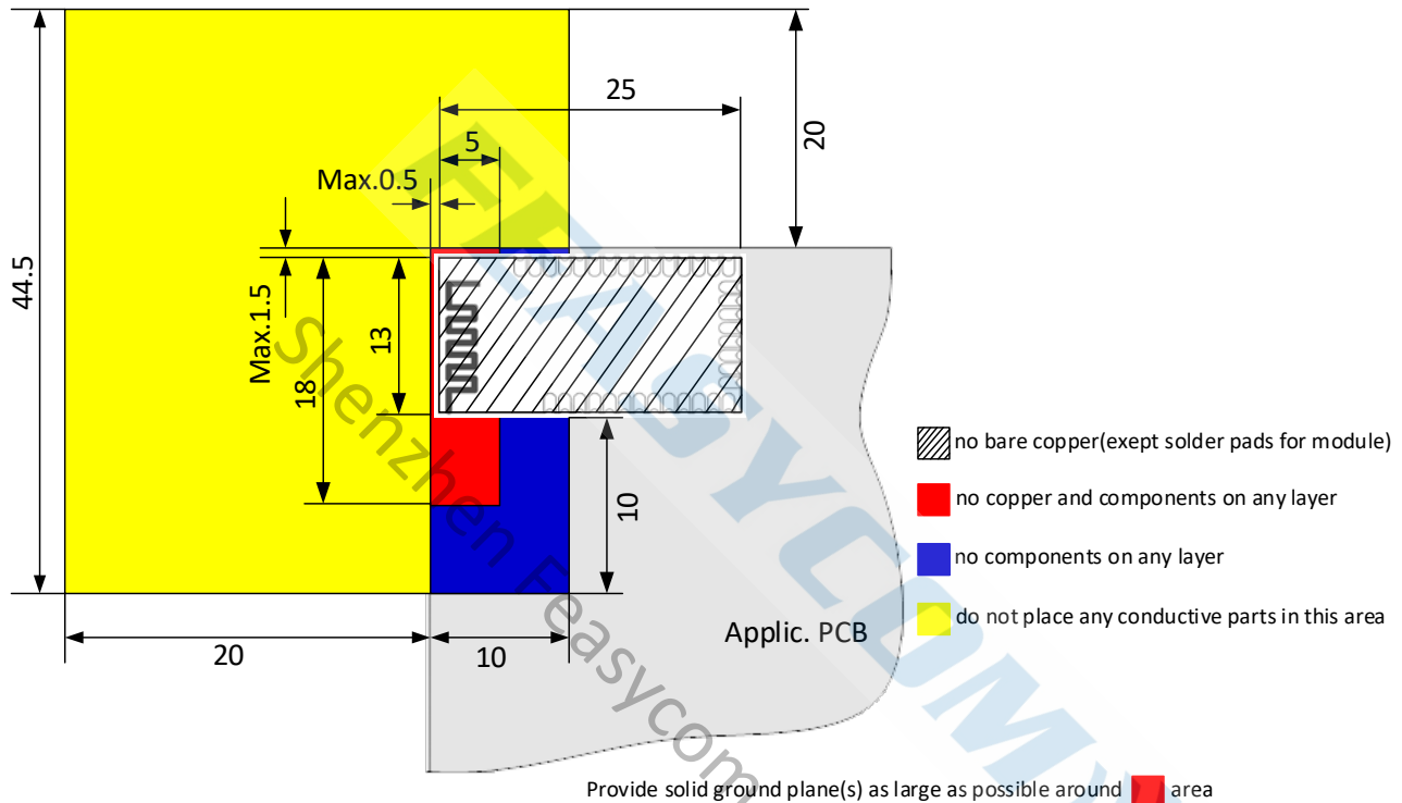
Figure 13: FSC-BT618V Restricted Area (Unit: mm)
