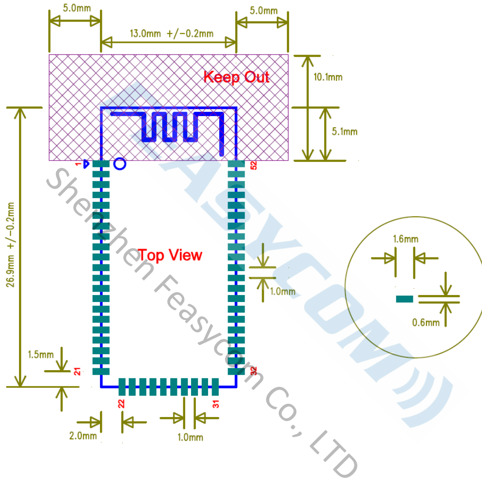
Figure 7: FSC-BT955 footprint
