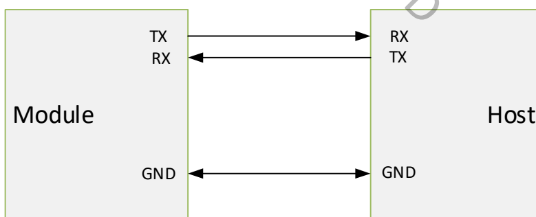
Figure 4: UART Connection
