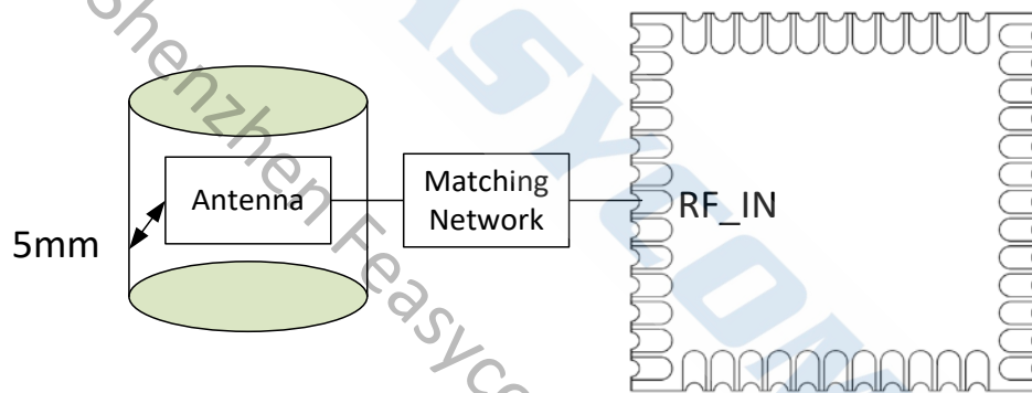
Figure 36: Leave 5mm Clearance Space from the Antenna
