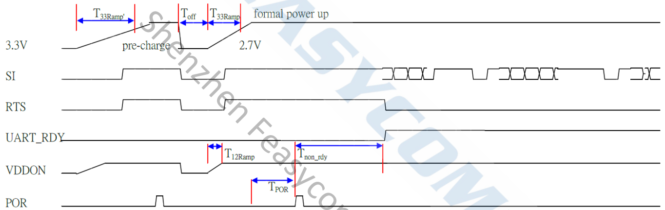
Figure 7: UART Power-On Sequence Without Hardware Flow Control
