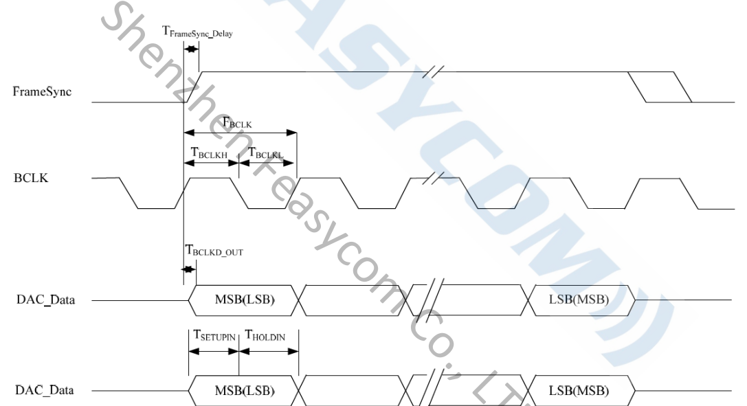
Figure 10: PCM interface timing (Long FrameSync)
