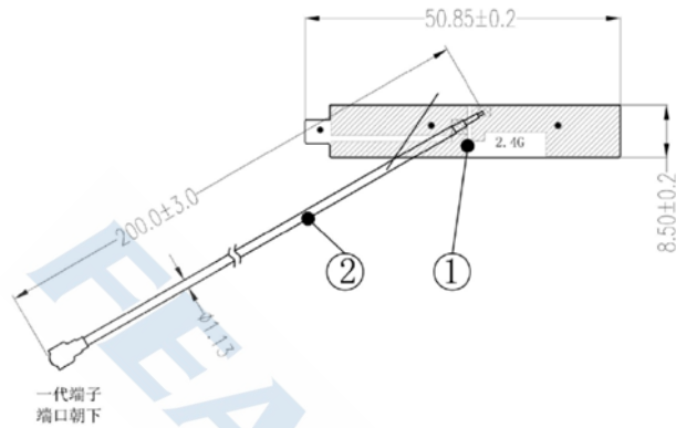
Figure 39: 2.4GHz antenna with IPEX first generation interface
